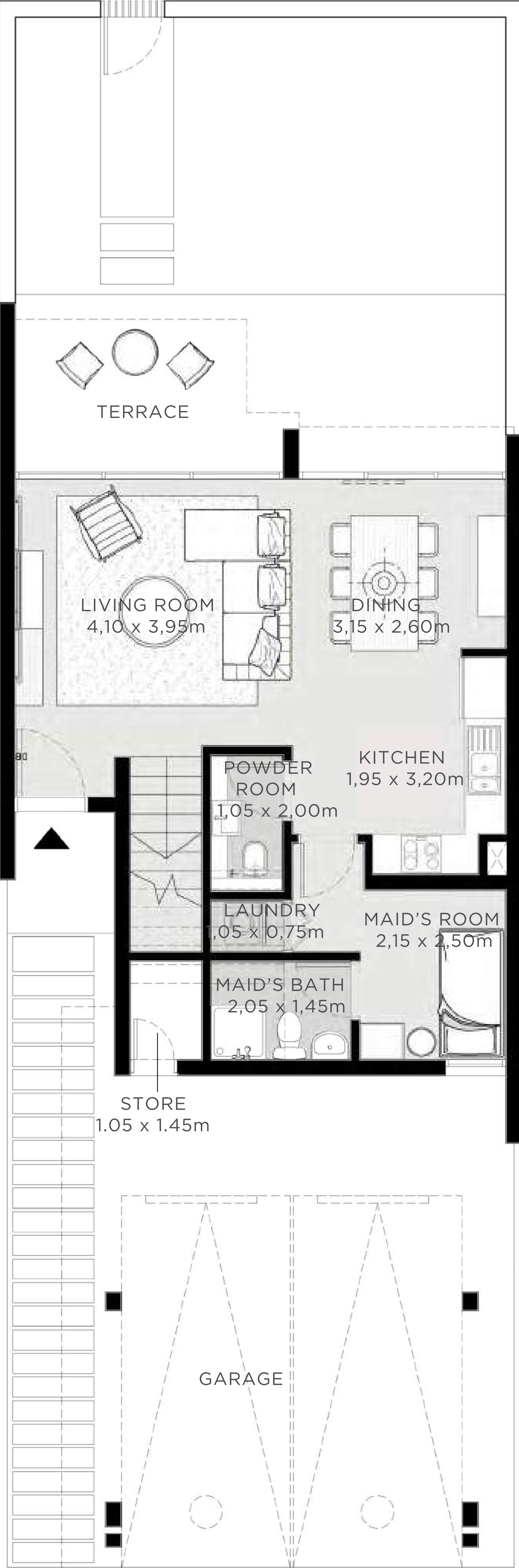
GROUND FLOOR
