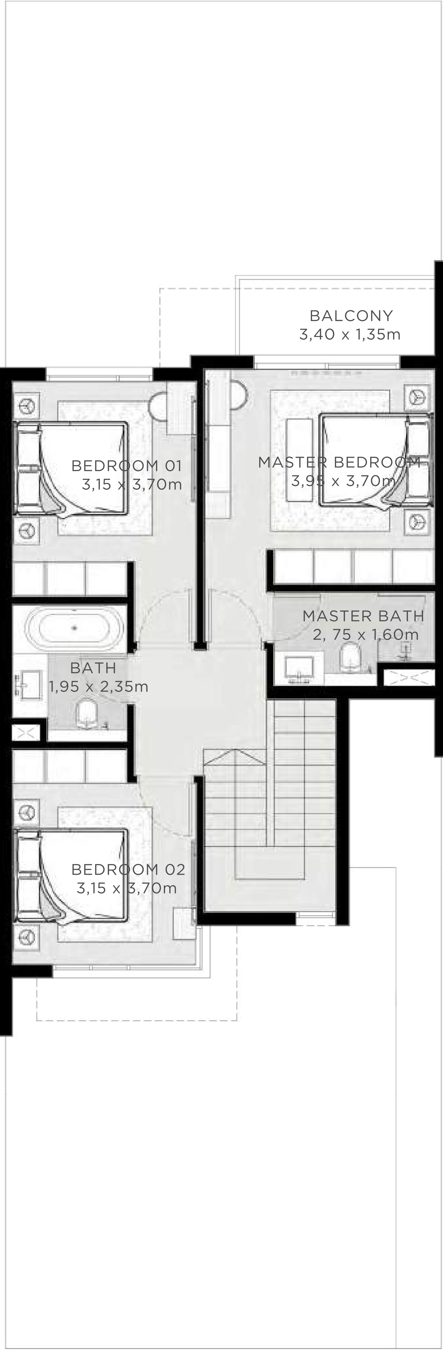
FIRST FLOOR
