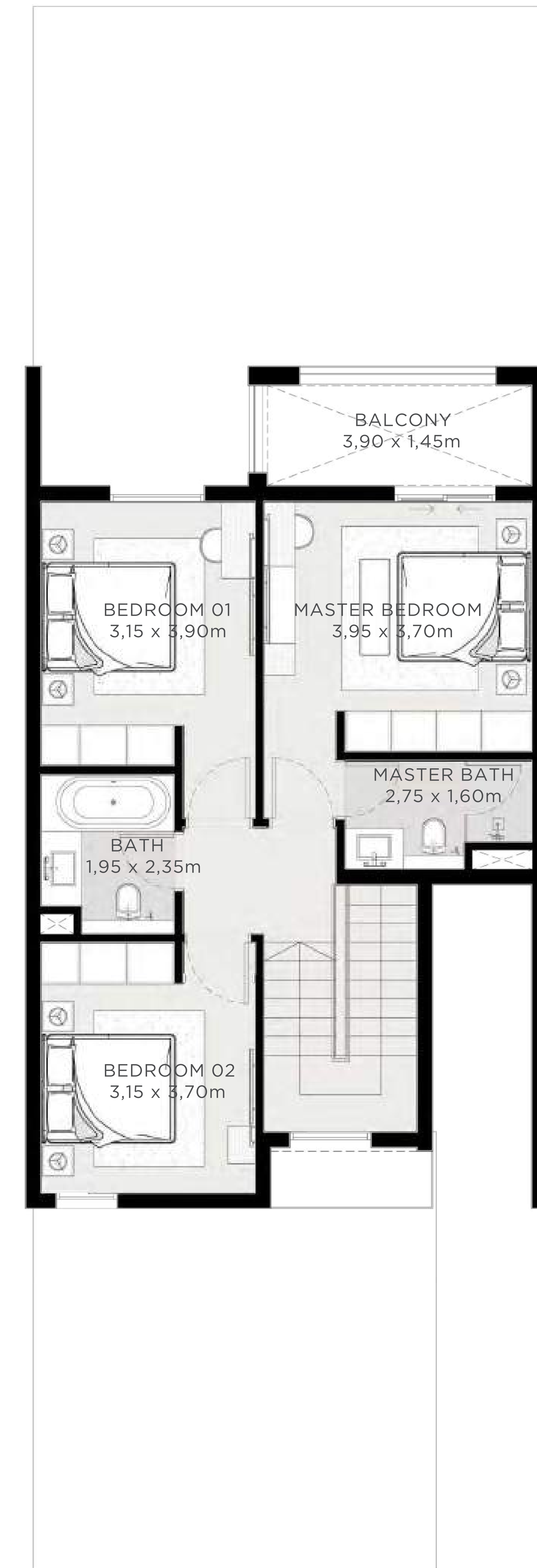
FIRST FLOOR
