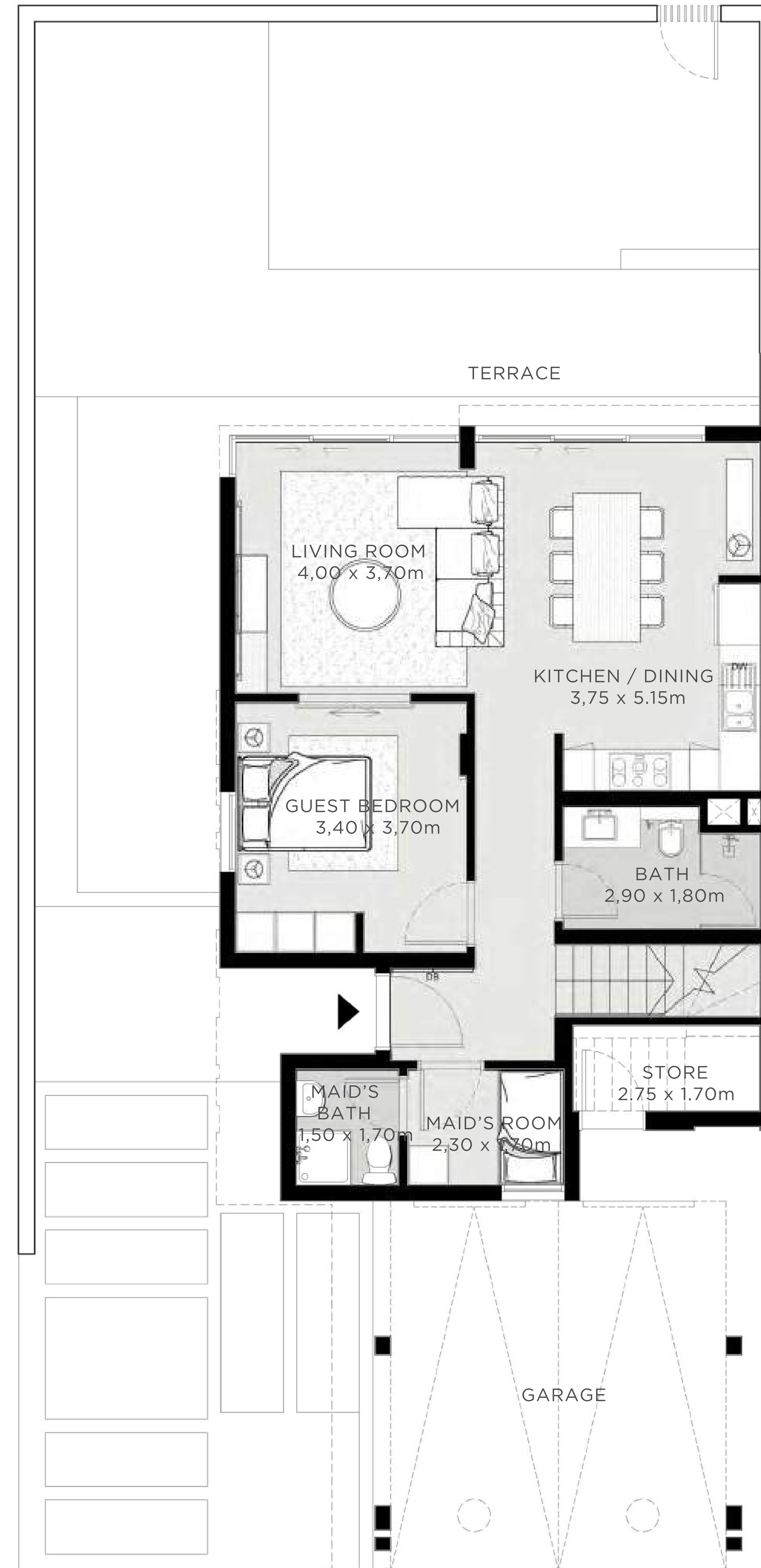
GROUND FLOOR
