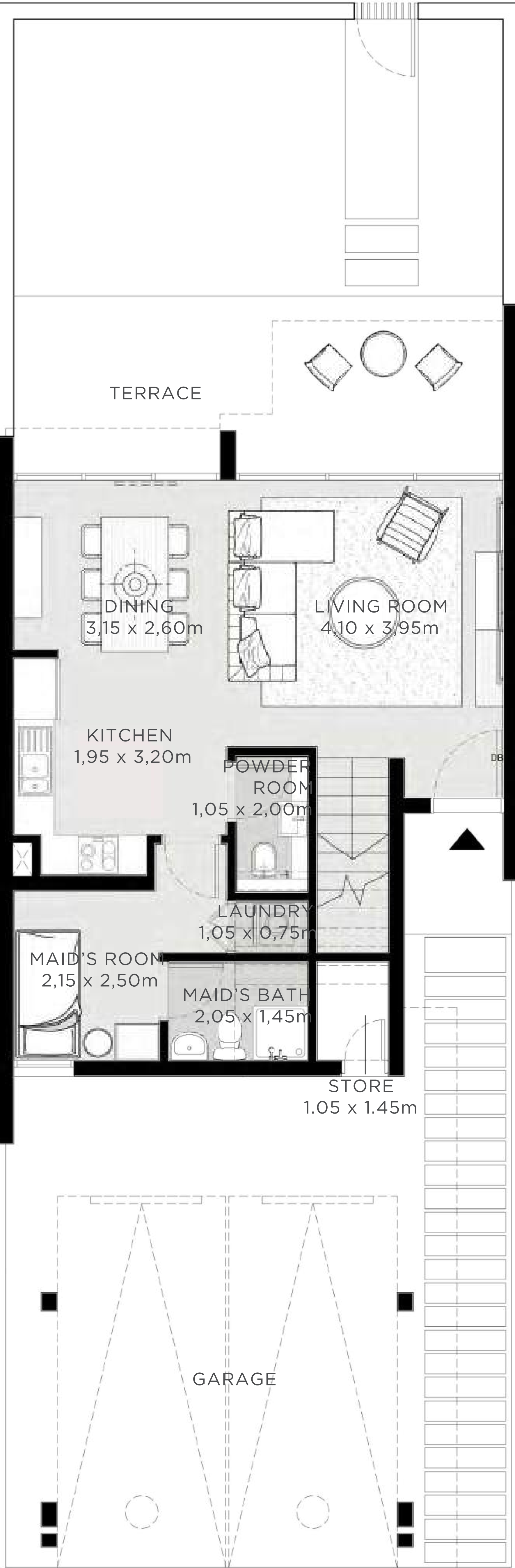
GROUND FLOOR
